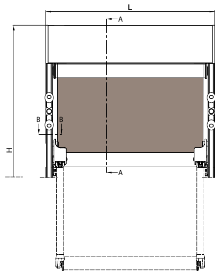
vista posteriore - rear view
